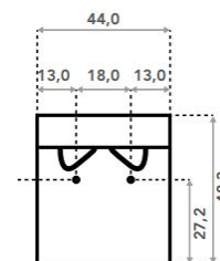
B(Din-rail),
